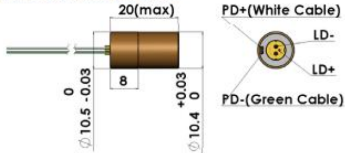
Dimensions and Pin Configuration (Unit: mm)
